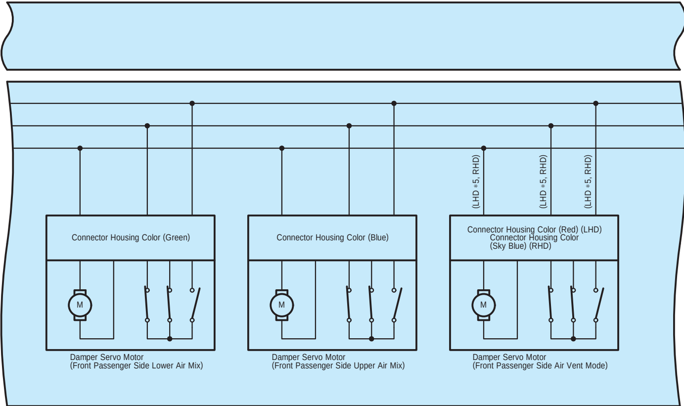
z1(C) Air Conditioner Harness Assembly
