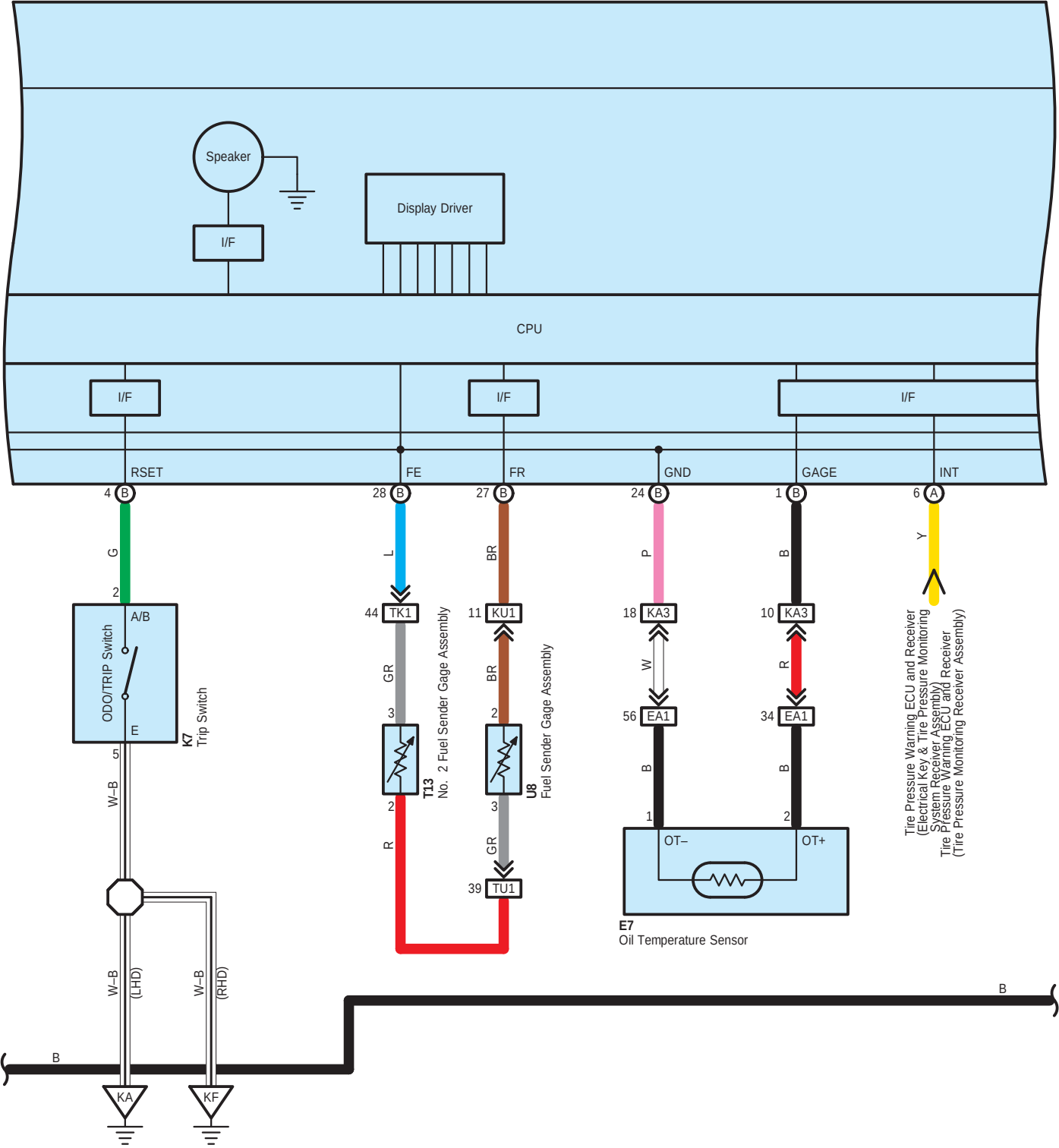
K32(A), K33(B), K120(C) Combination Meter Assembly
