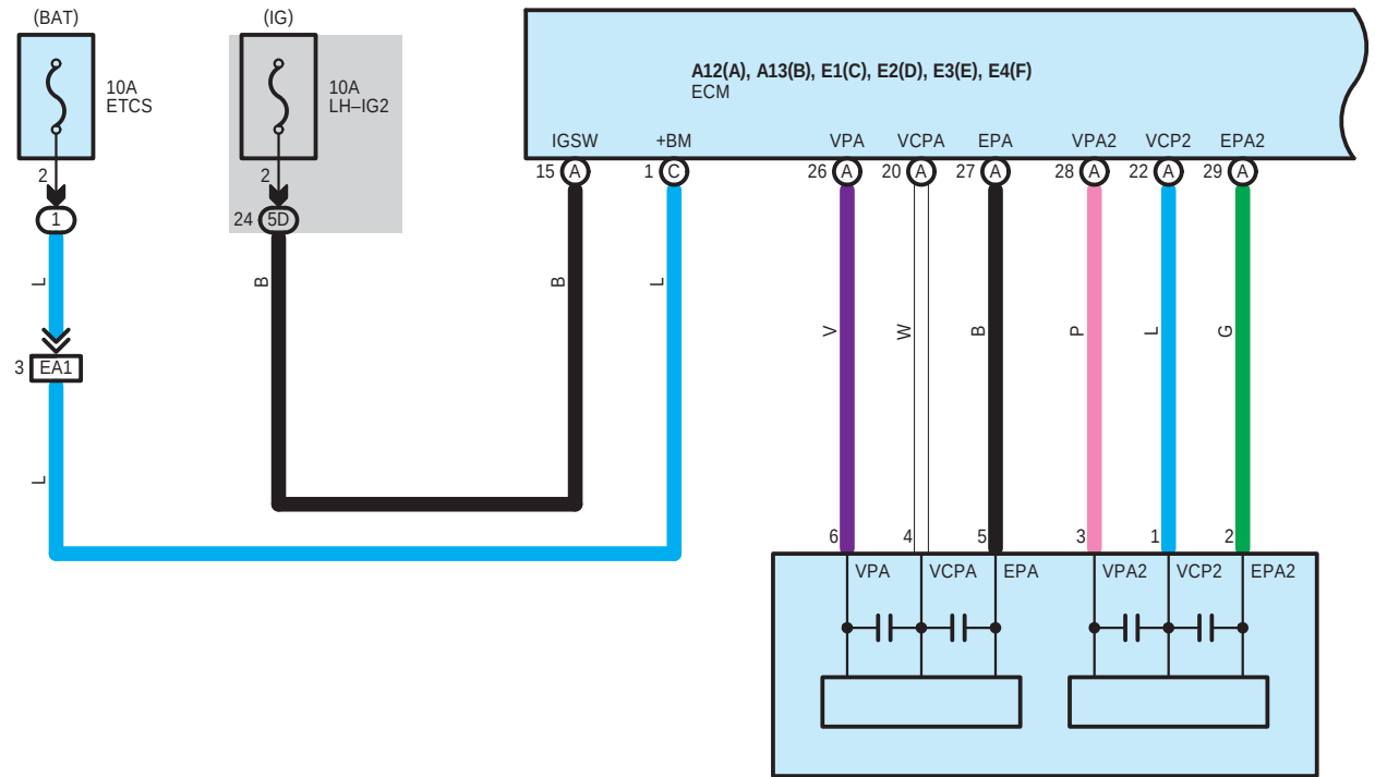
A1 Accelerator Pedal Sensor Assembly
