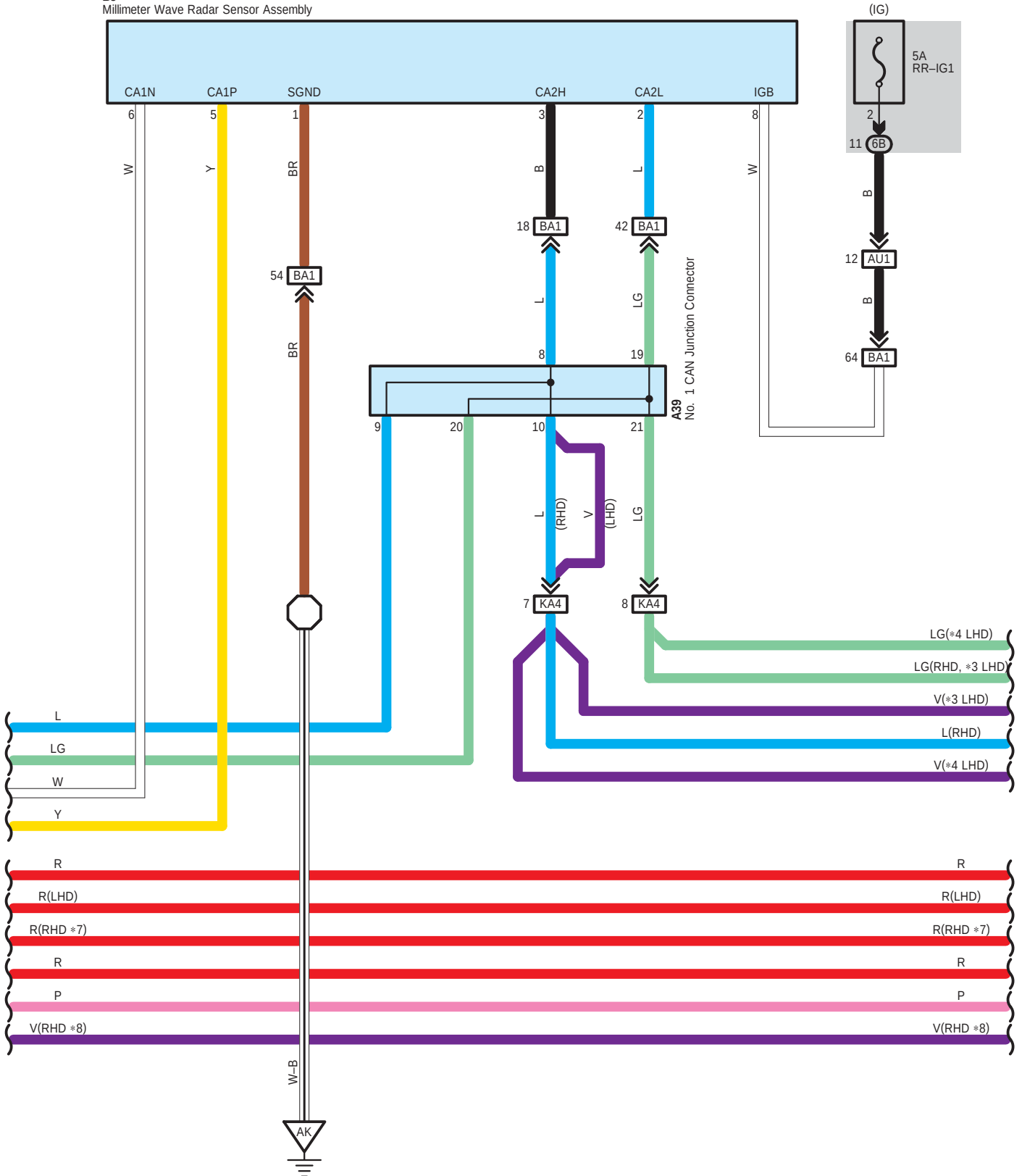
B5 Millimeter Wave Radar Sensor Assembly
