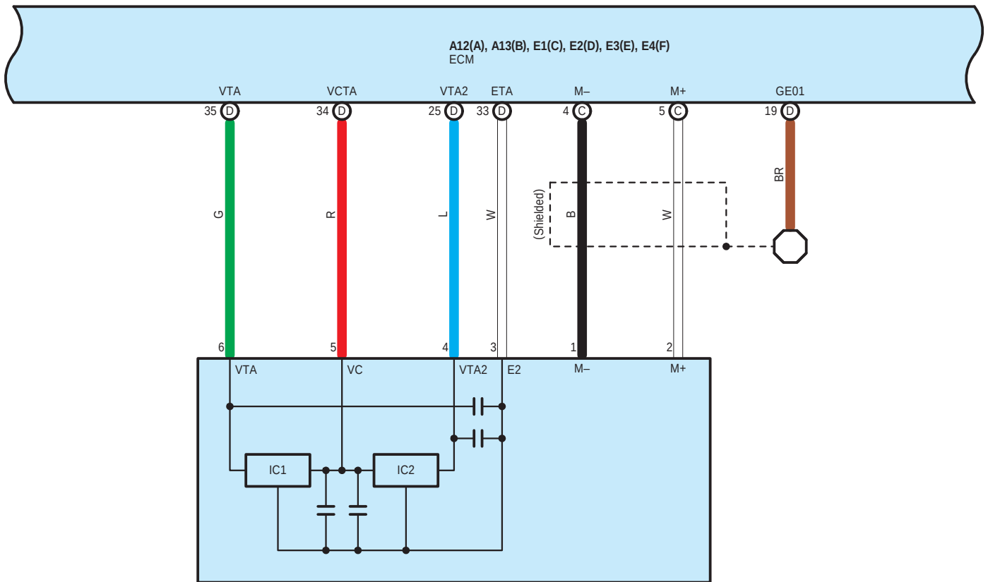
E36 Throttle Body with Motor Assembly
