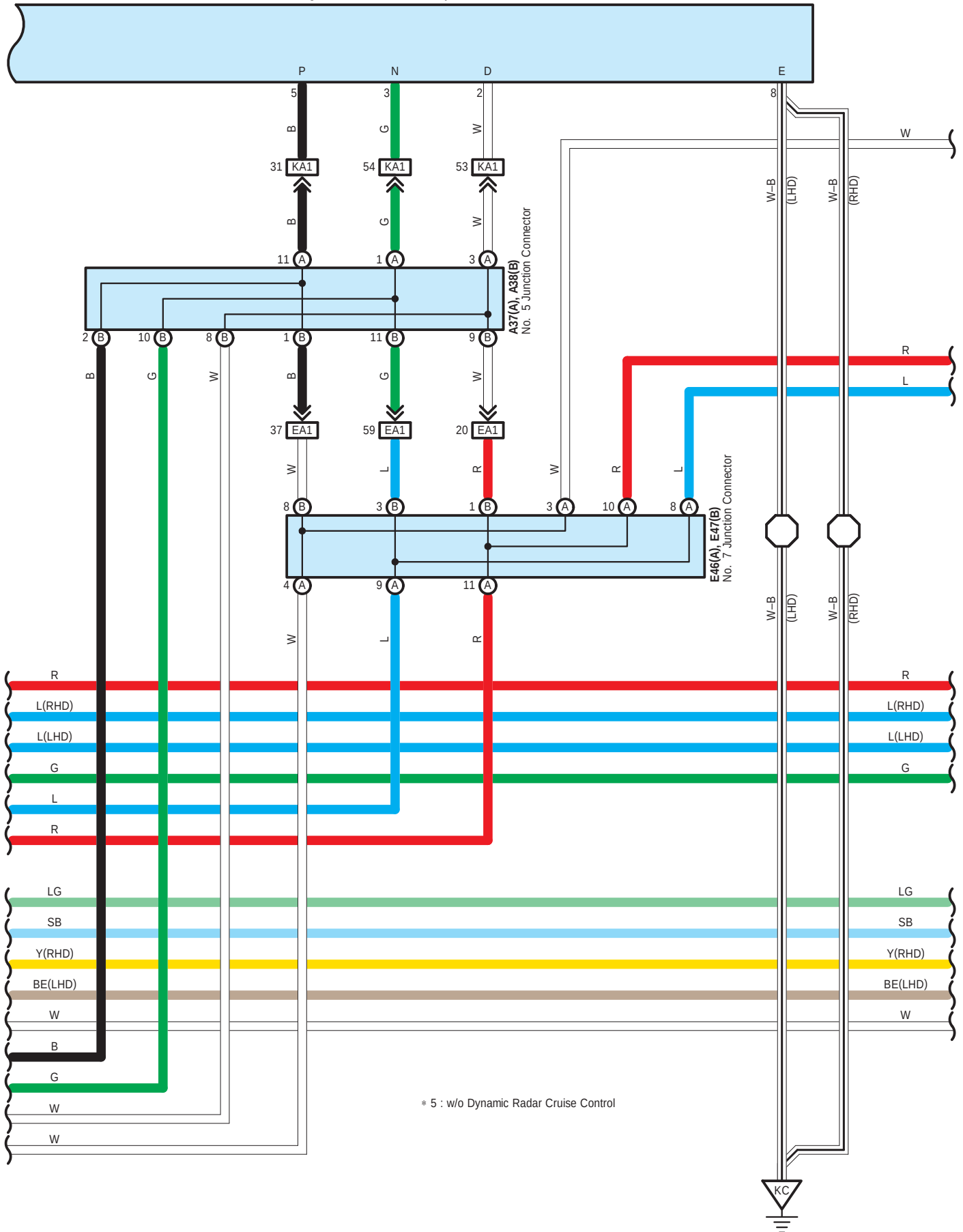
K49 A/T Shift Position Indicator (Shifting Hole Frame Sub-Assembly)
