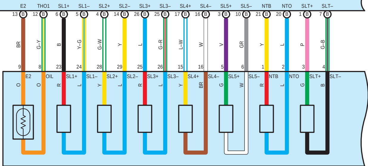
E24 Electronically Controlled Transmission Solenoid (Transmission Wire)
