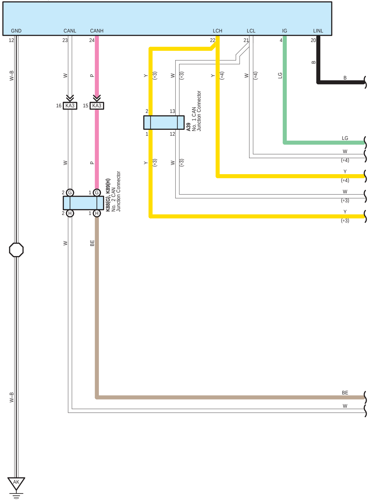
A29 Headlight Light Control ECU Sub-Assembly LH
