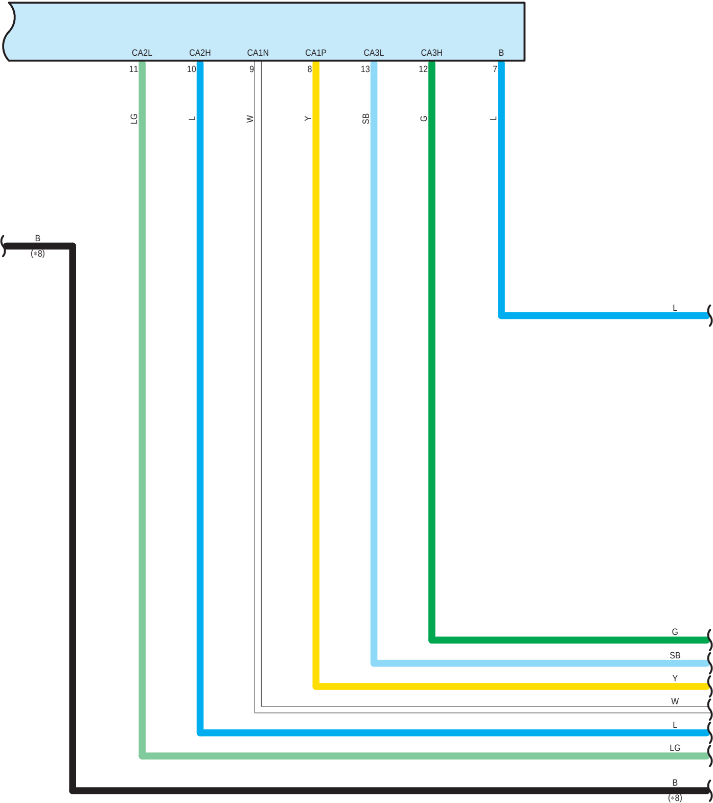
K4 Driving Support ECU Assembly
