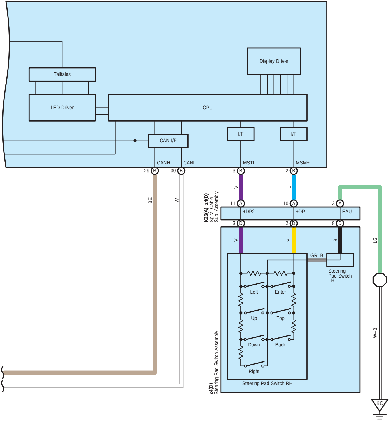
K33(B) Combination Meter Assembly
