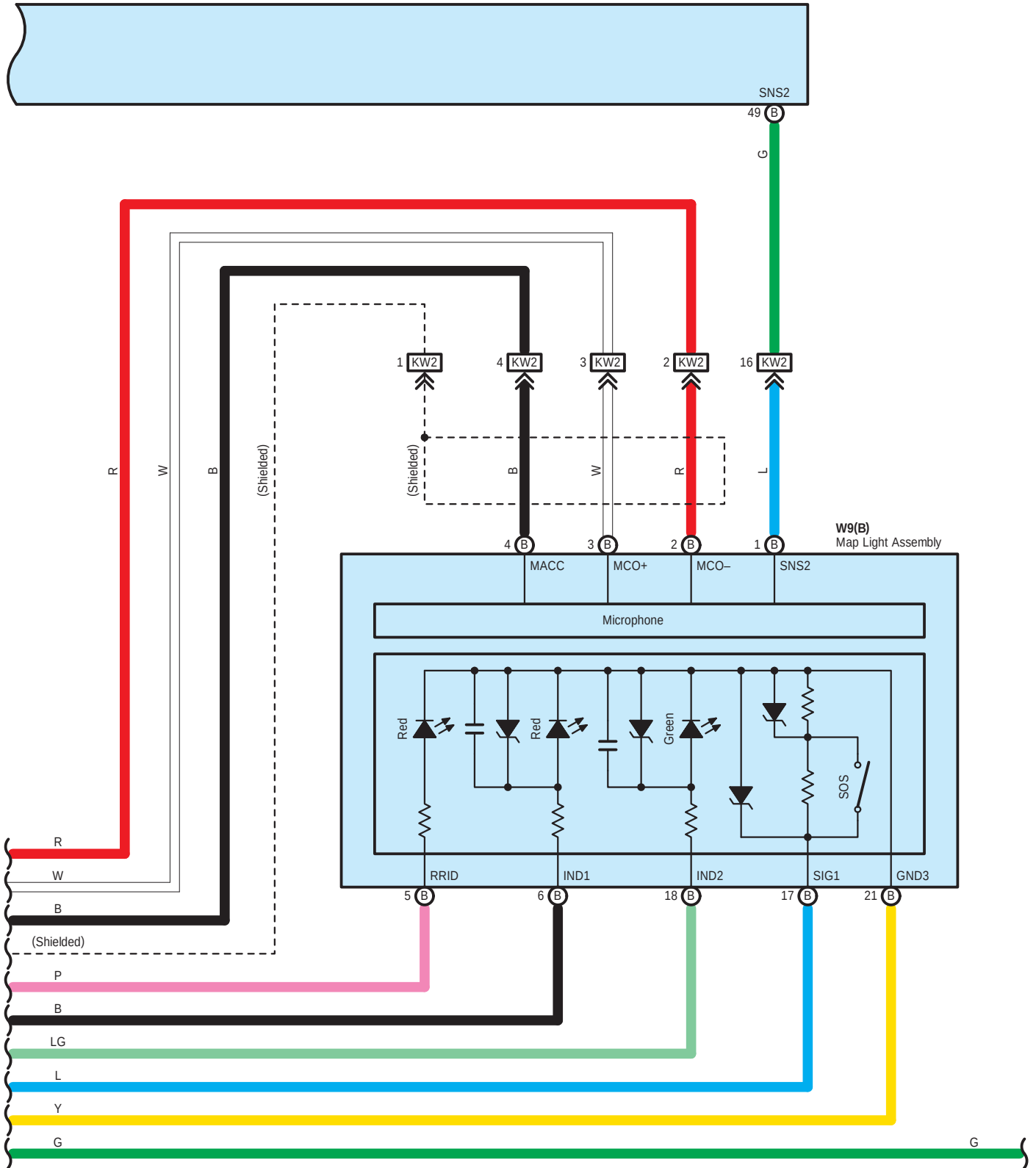
K57(B) Radio Receiver Assembly
