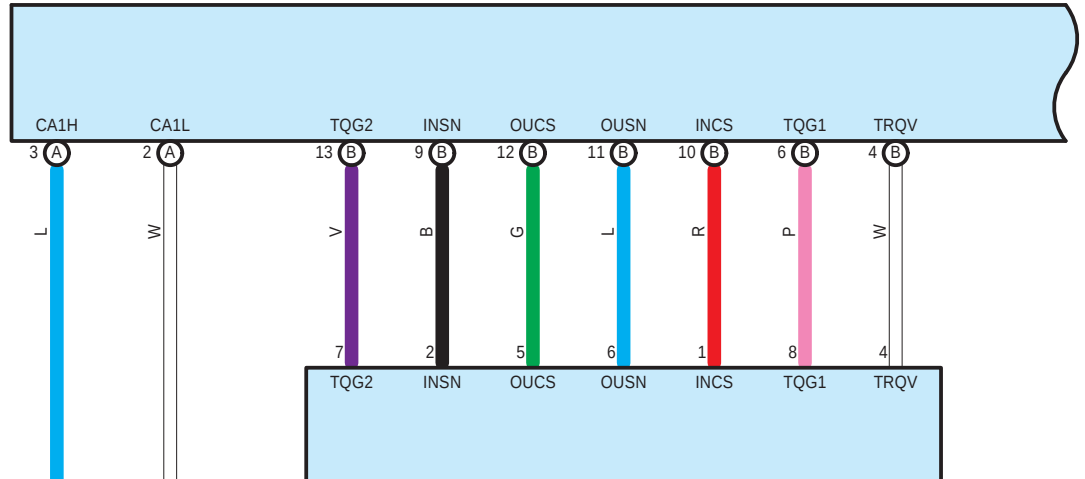
C3 Power Steering Torque Sensor (Power Steering Link Assembly)
