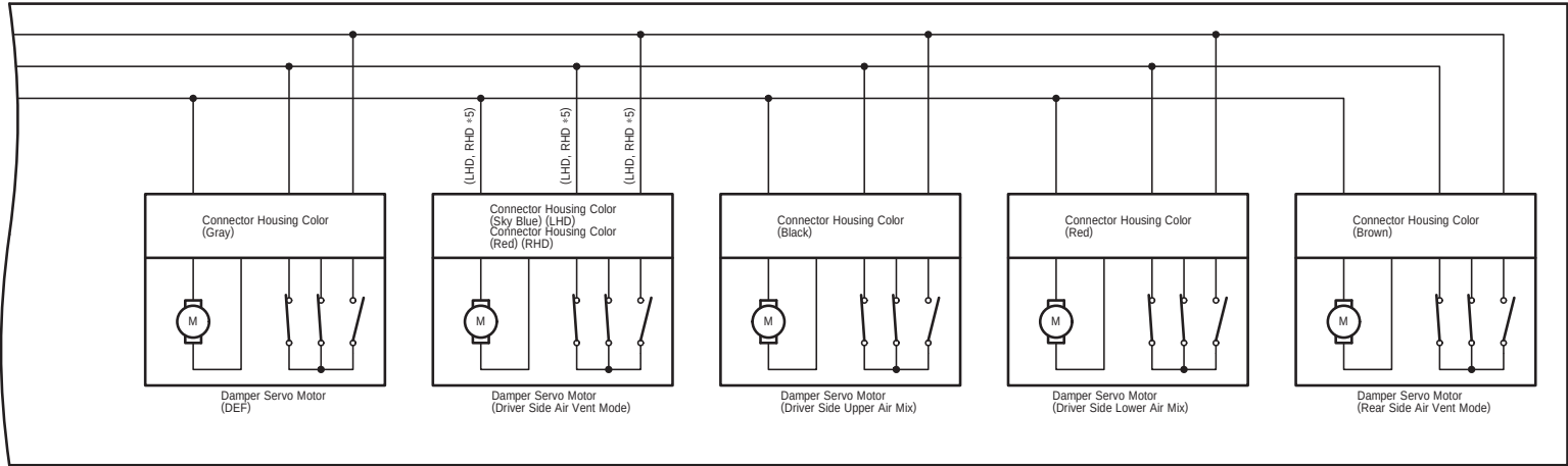
z1(C) A/C Harness Assembly
