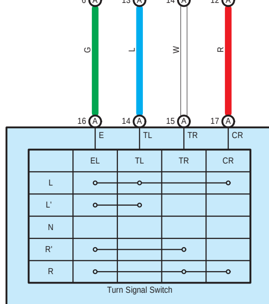
N28(A) Headlight Dimmer Switch Assembly
