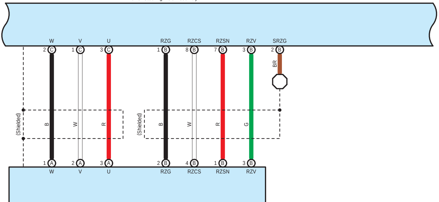
C1(A), C2(B) Power Steering Motor (Power Steering Link Assembly)
