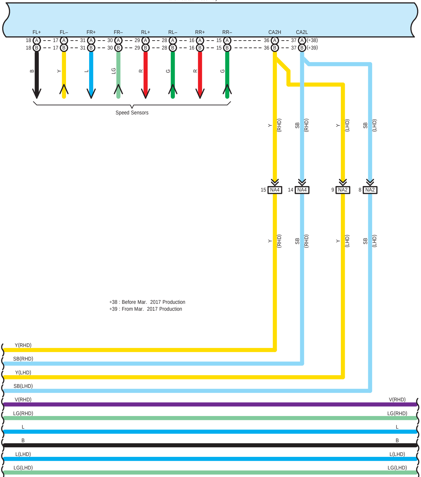
A77(A), A94(B) Brake Actuator Assembly
