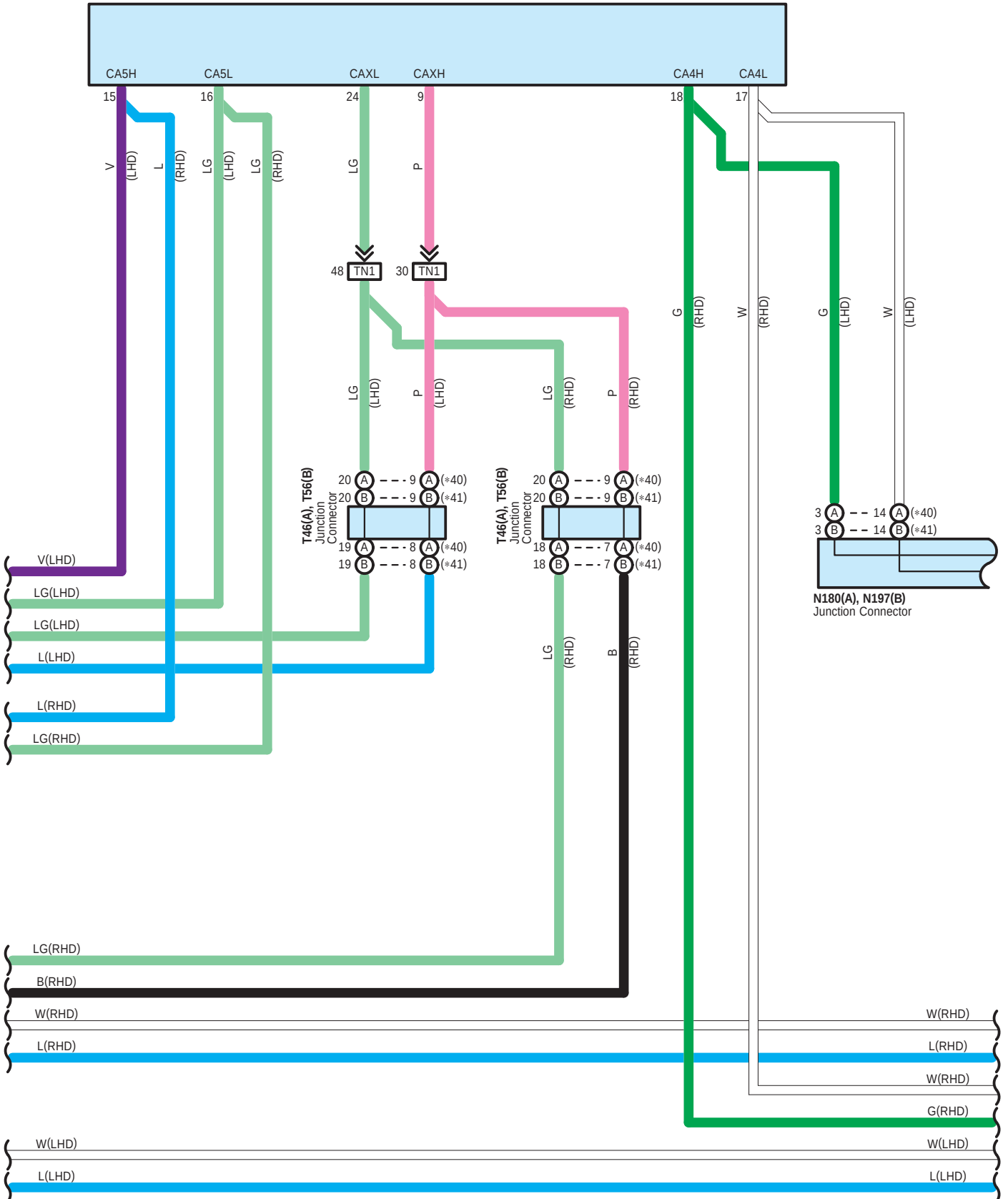
N176 Network Gateway ECU
