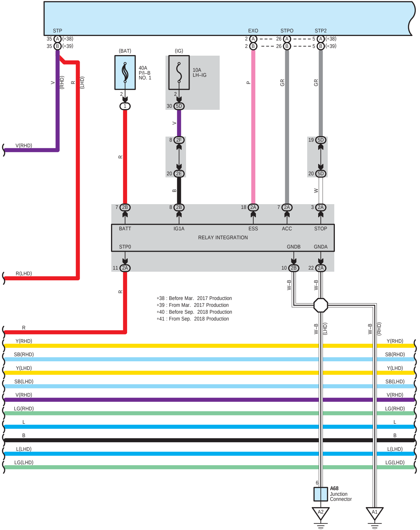
A77(A), A94(B) Brake Actuator Assembly
