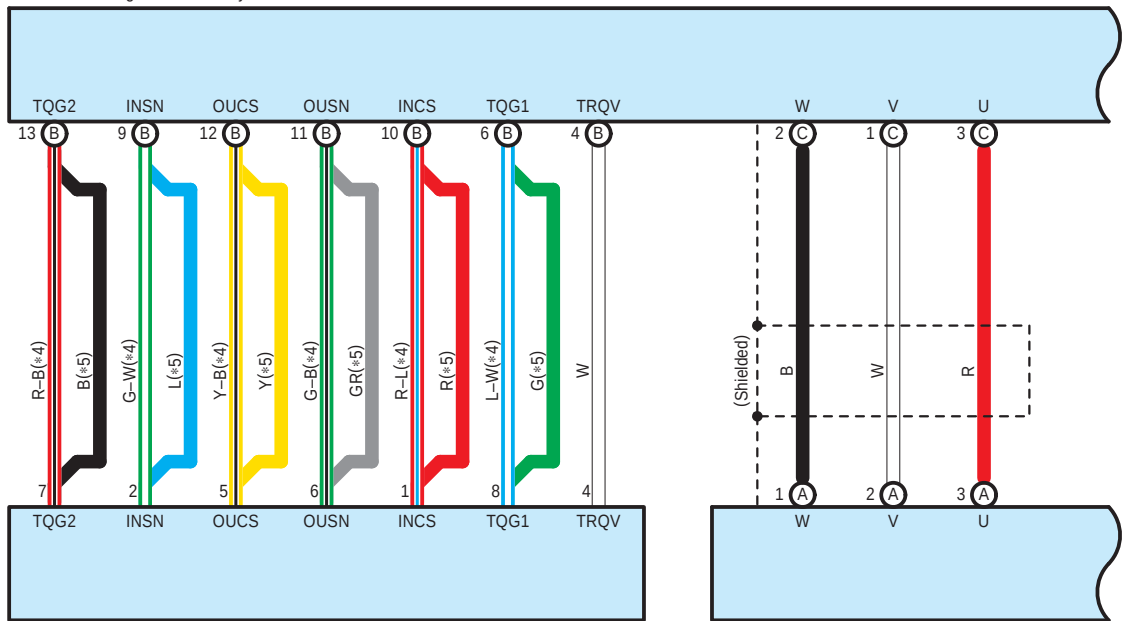
C3 Power Steering Torque Sensor (Power Steering Link Assembly)
