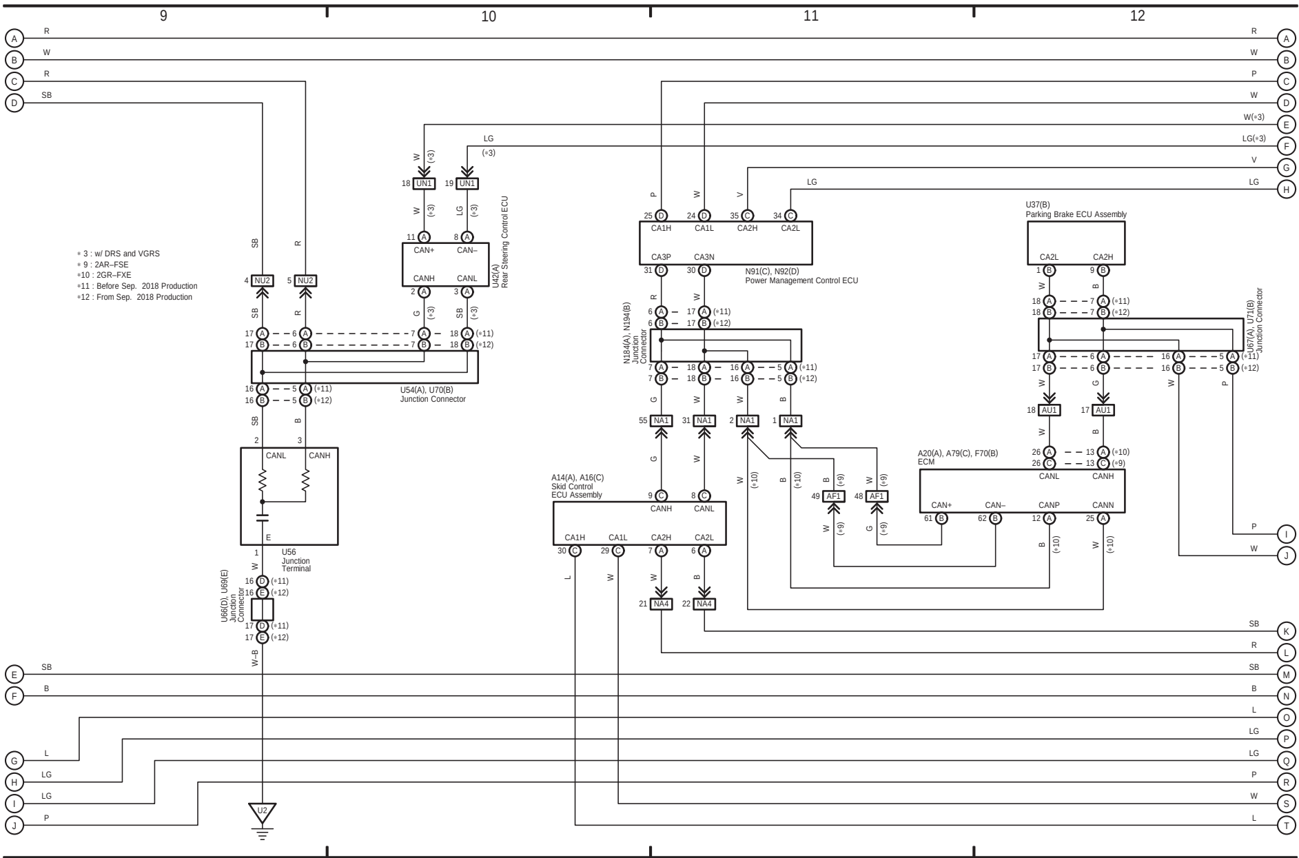
Multiplex Communication System (CAN LHD) (From Oct. 2015 Production)
