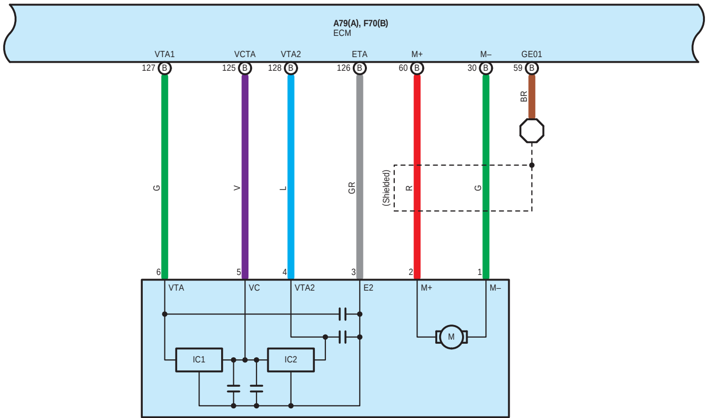
F24 Throttle Body with Motor Assembly
