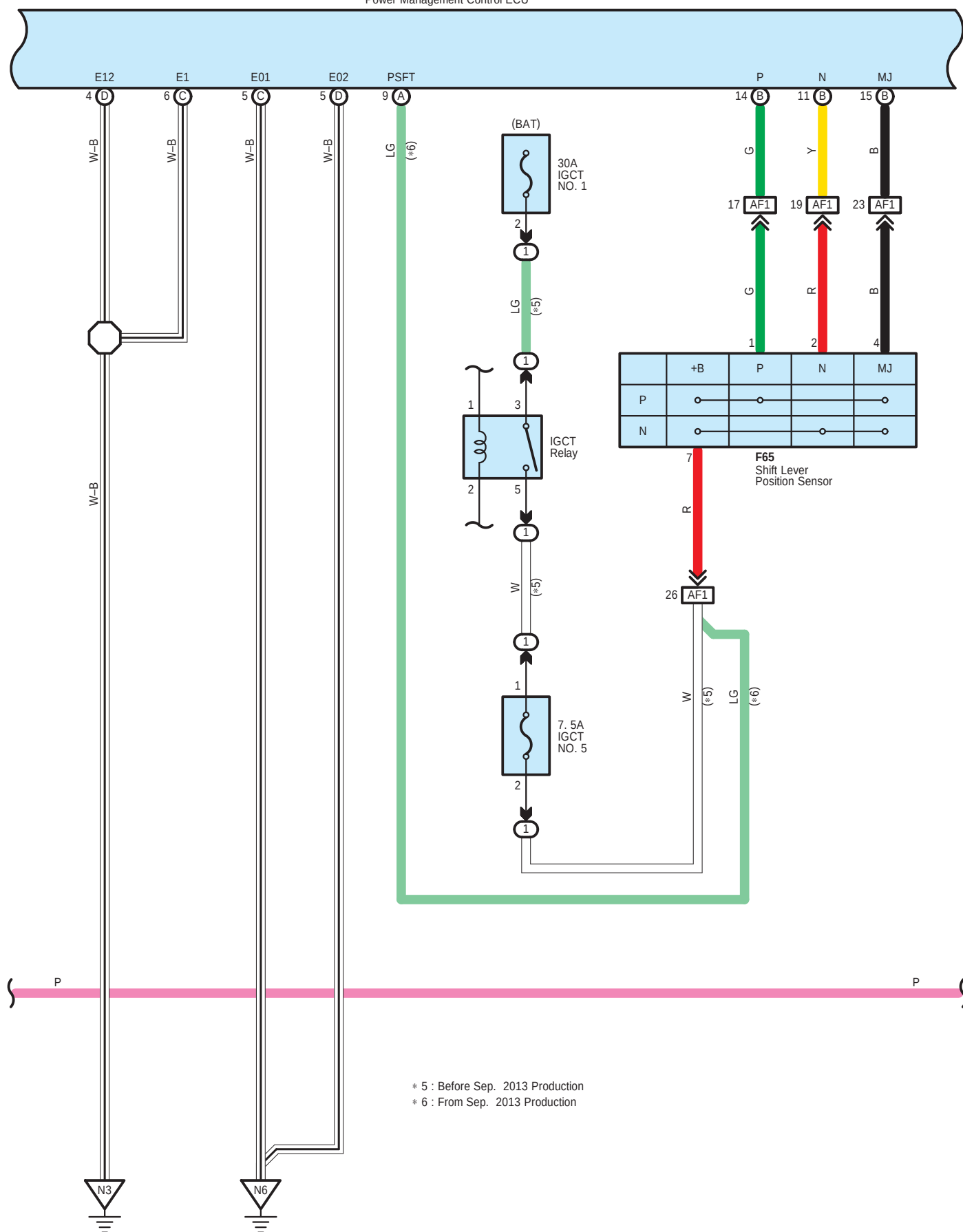
A35(A), A36(B), N91(C), N92(D) Power Management Control ECU
