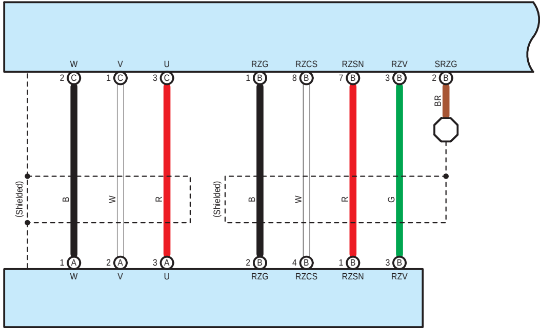
C1(A), C2(B) Power Steering Motor (Power Steering Link Assembly)
