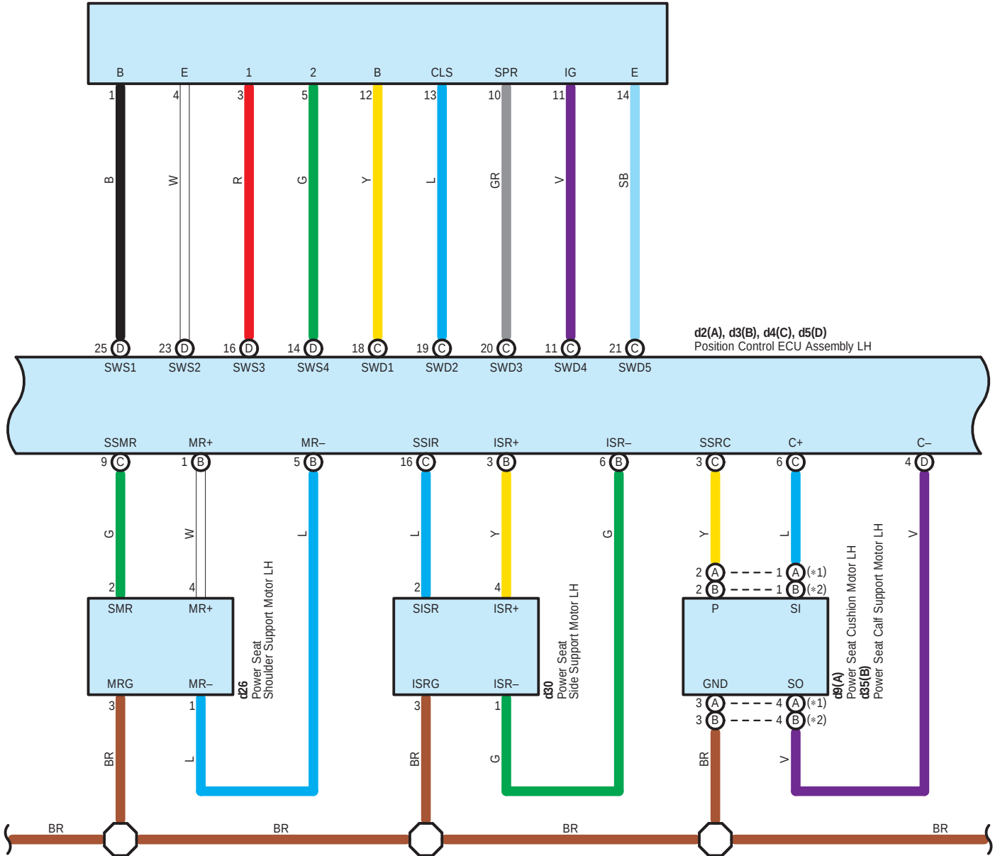
d18 Front Power Seat Switch Assembly LH
