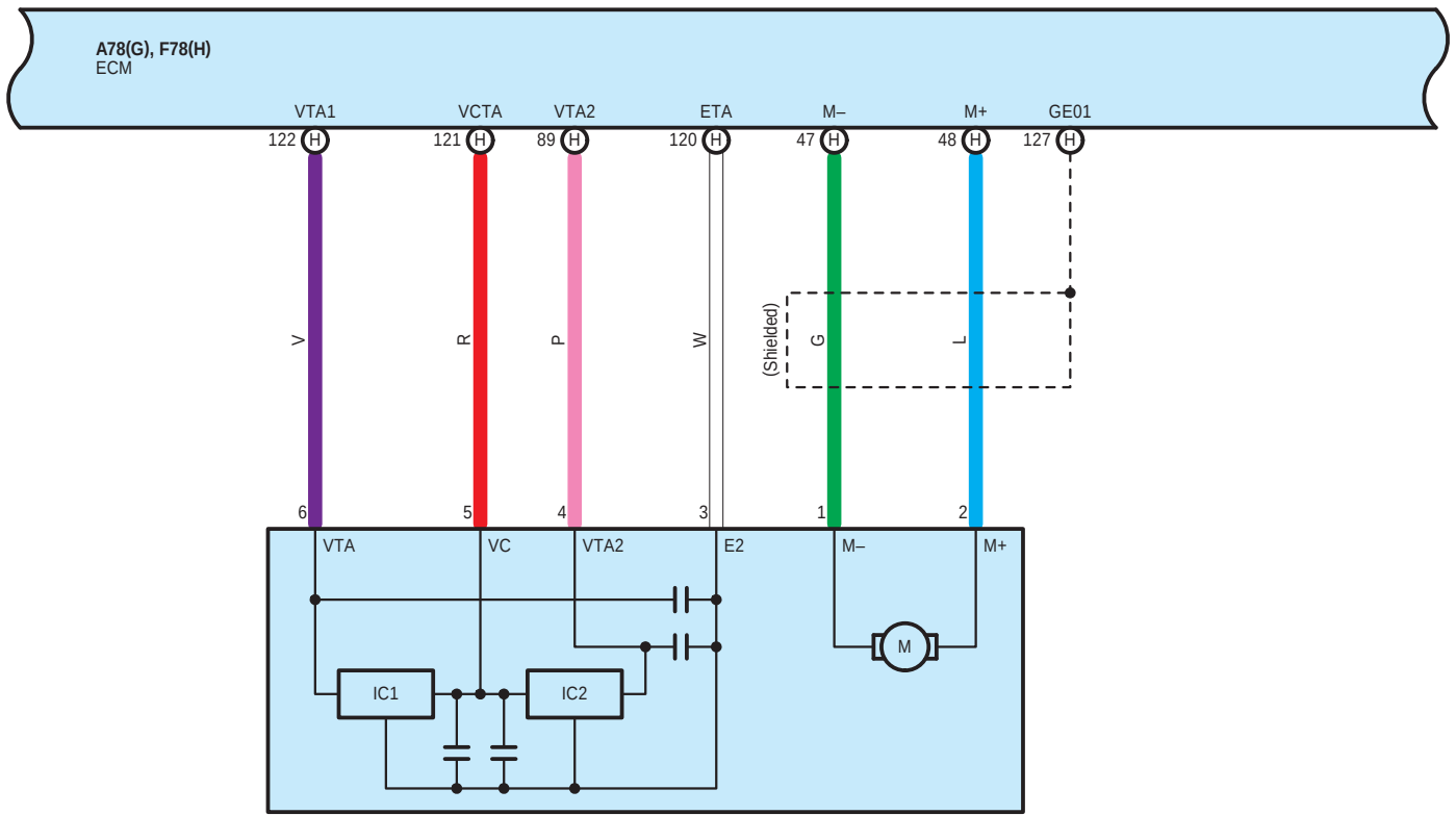
F24 Throttle Body Assembly with Motor
