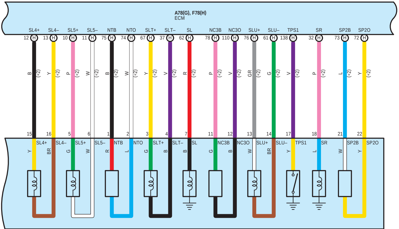
F73 ECT Solenoid (Transmission Wire)
