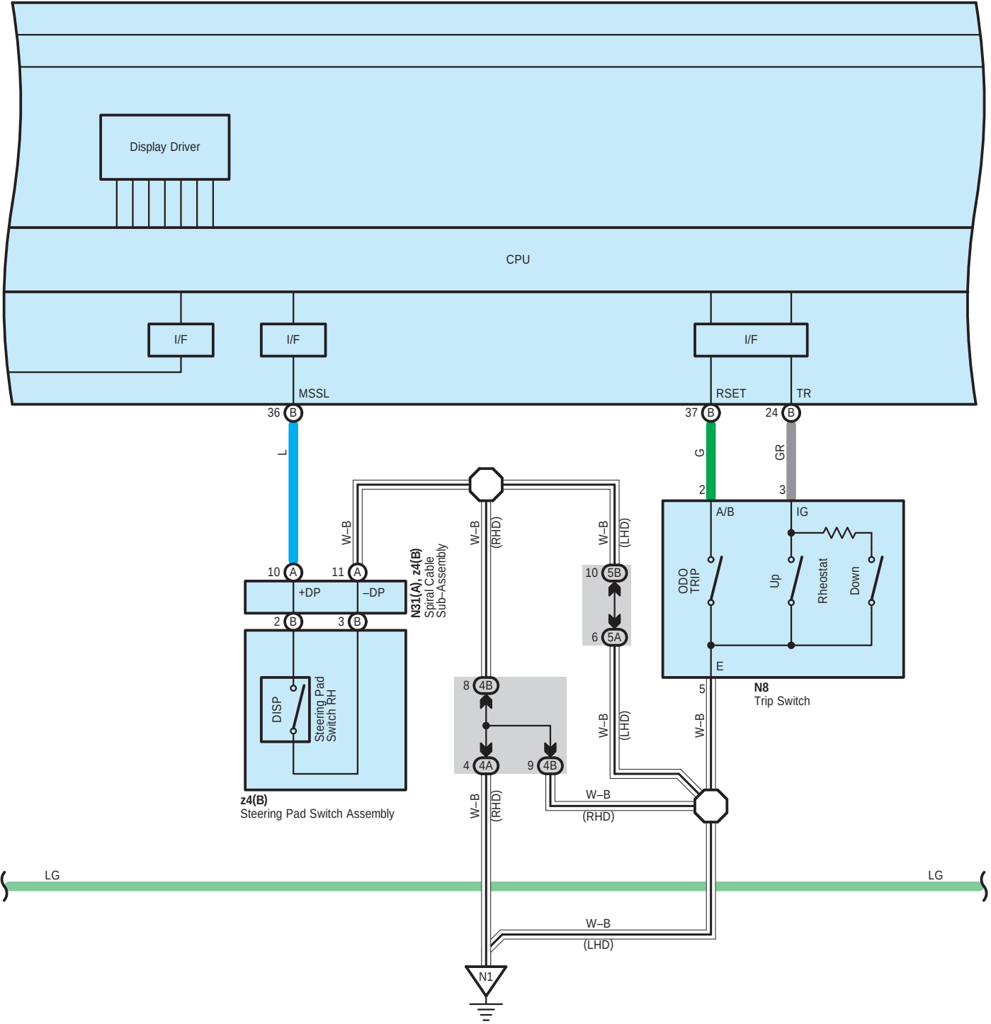
N39(A), N40(B) Combination Meter Assembly
