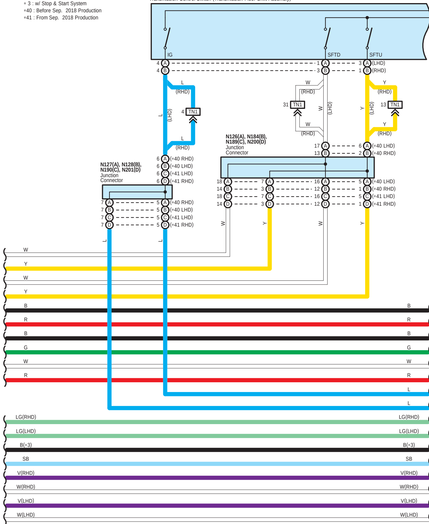
N50(A), T11(B) Transmission Control Switch (Transmission Floor Shift Assembly)
