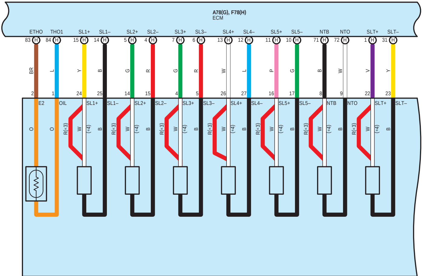
F73 ECT Solenoid (Transmission Wire)
