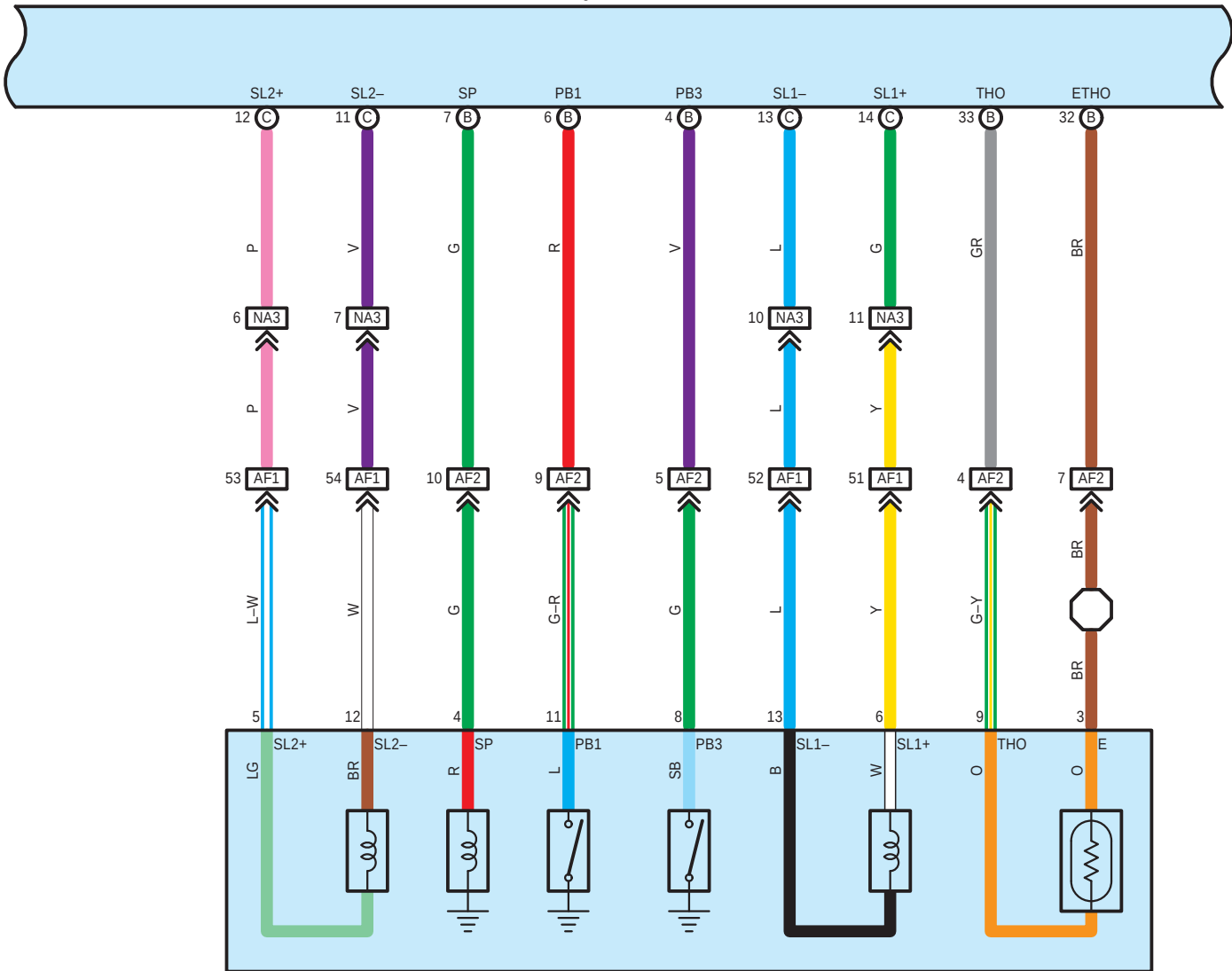
F52 Hybrid Vehicle Transmission (Transmission Wire)
