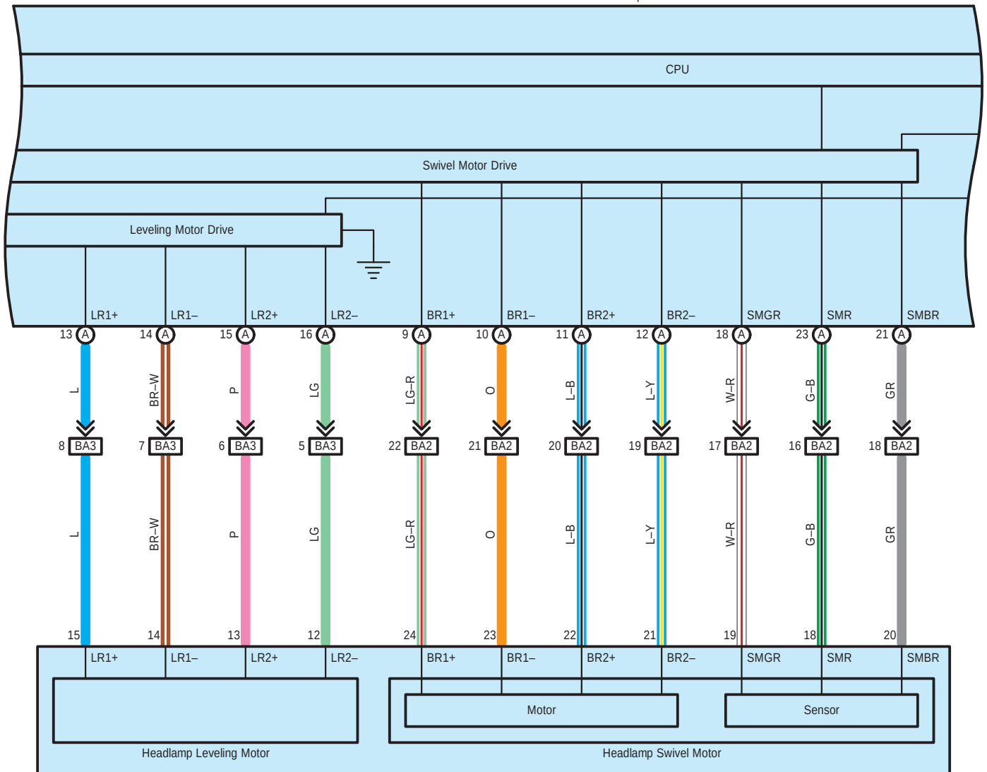
B2 Headlamp Assembly (RH)
