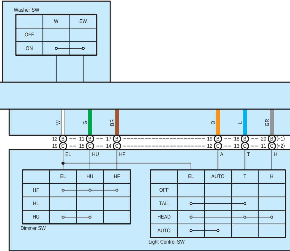
z3(B), (C) Headlamp Dimmer SW Assembly
