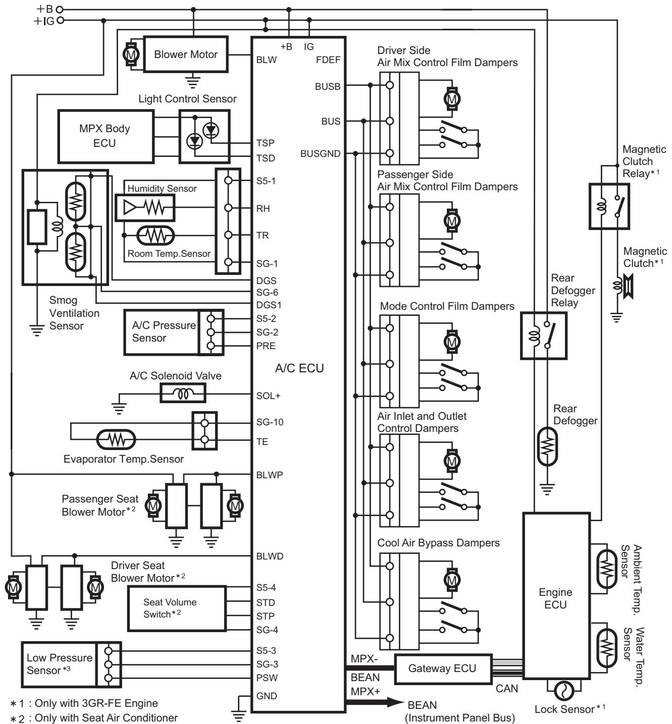
Automatic Air conditioner System Diagram
