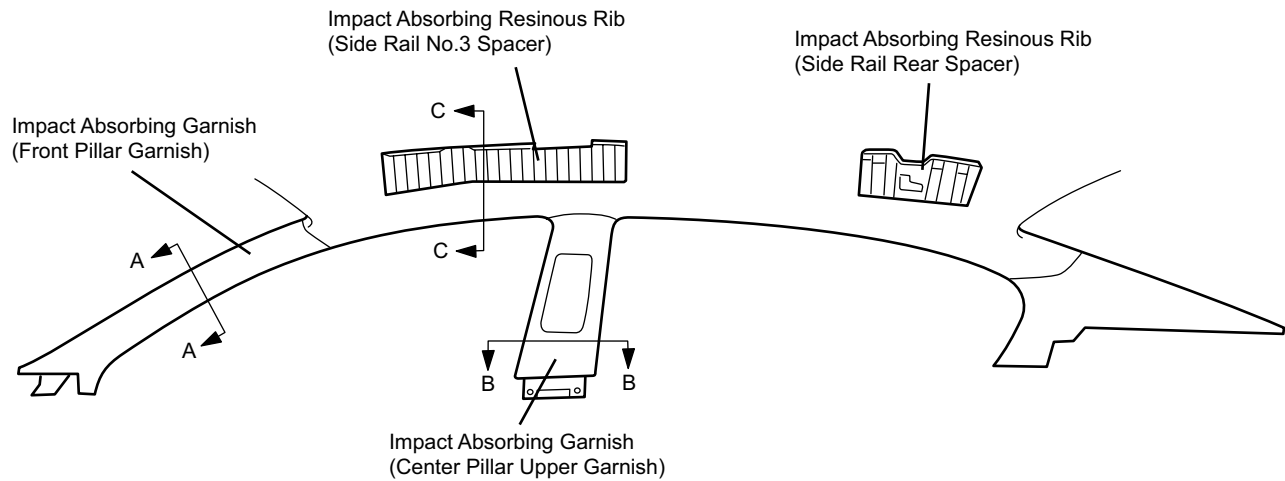
Shock absorbing section material position
