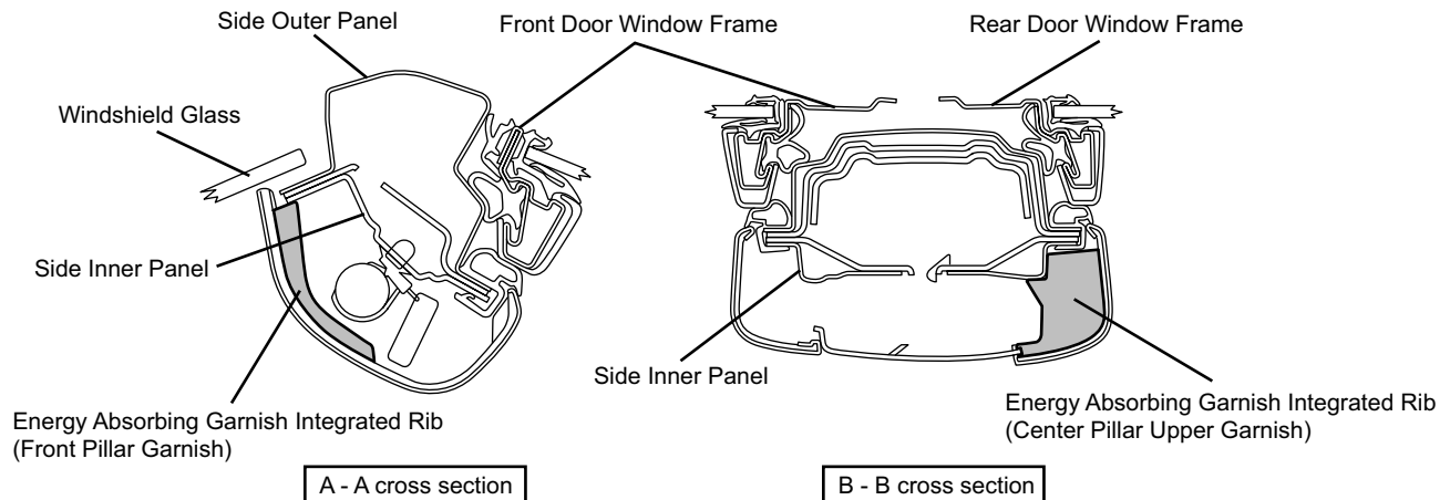
Energy Absorption Material Allocation (cross-sectional view)
