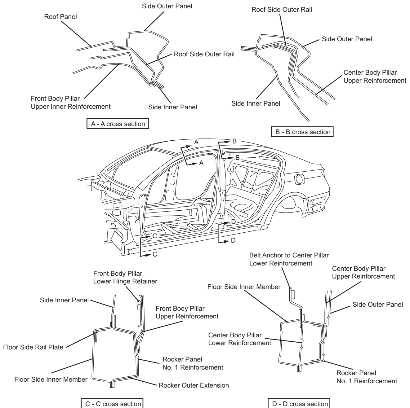
Panel Joint (cross-sectional view)
