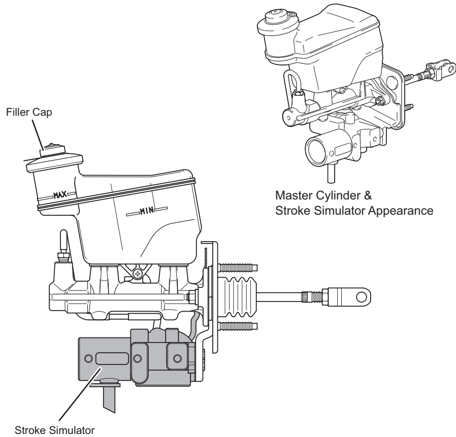
Master Cylinder & Stroke Simulator Side View
