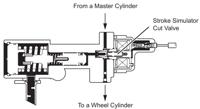
Stroke Simulator Cross Section
