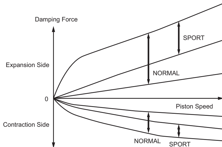
Attenuation Power Characteristic (Image)
