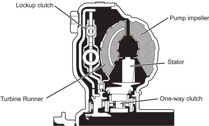
Torque converter (A760E)
