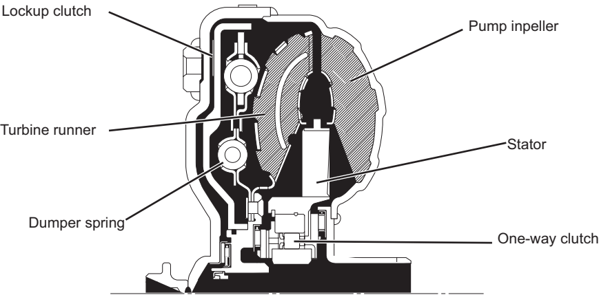
Torque converter (A761E)
