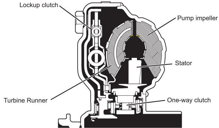
Torque converter (A960E)
