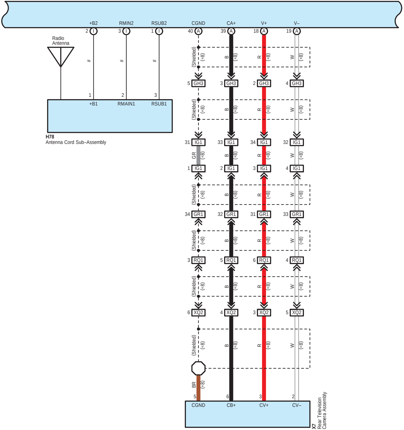
H45(A), H46(B), H47(C), H62(D), H64(E), H65(F), H69(G), H71(H), H77(I), H84(J) Multi-Media Module Receiver Assembly
