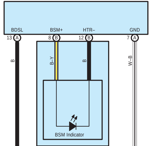
z3(B) Outer Rear View Mirror Assembly LH
