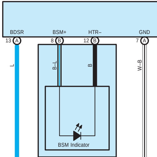
z2(B) Outer Rear View Mirror Assembly RH
