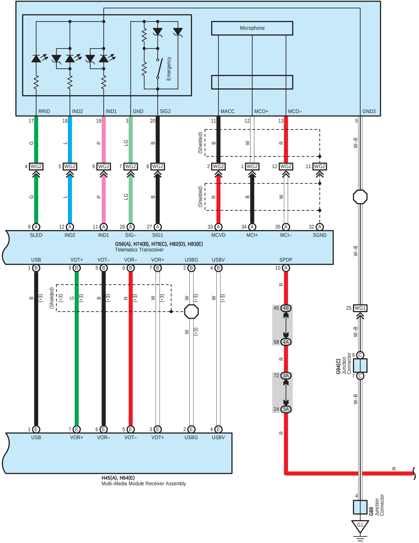
W7 Map Light Assembly
