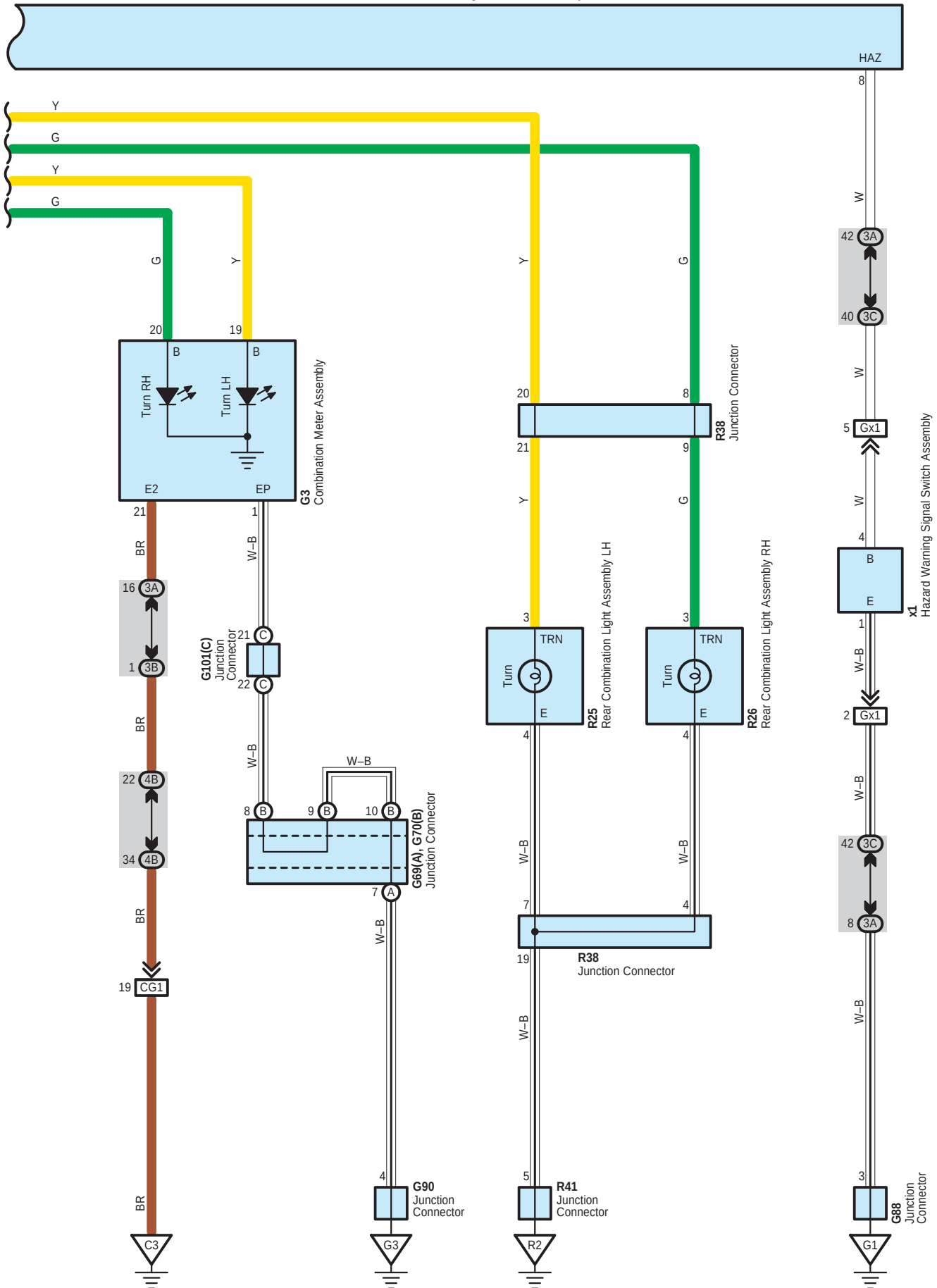
G4 Turn Signal Flasher Assembly
