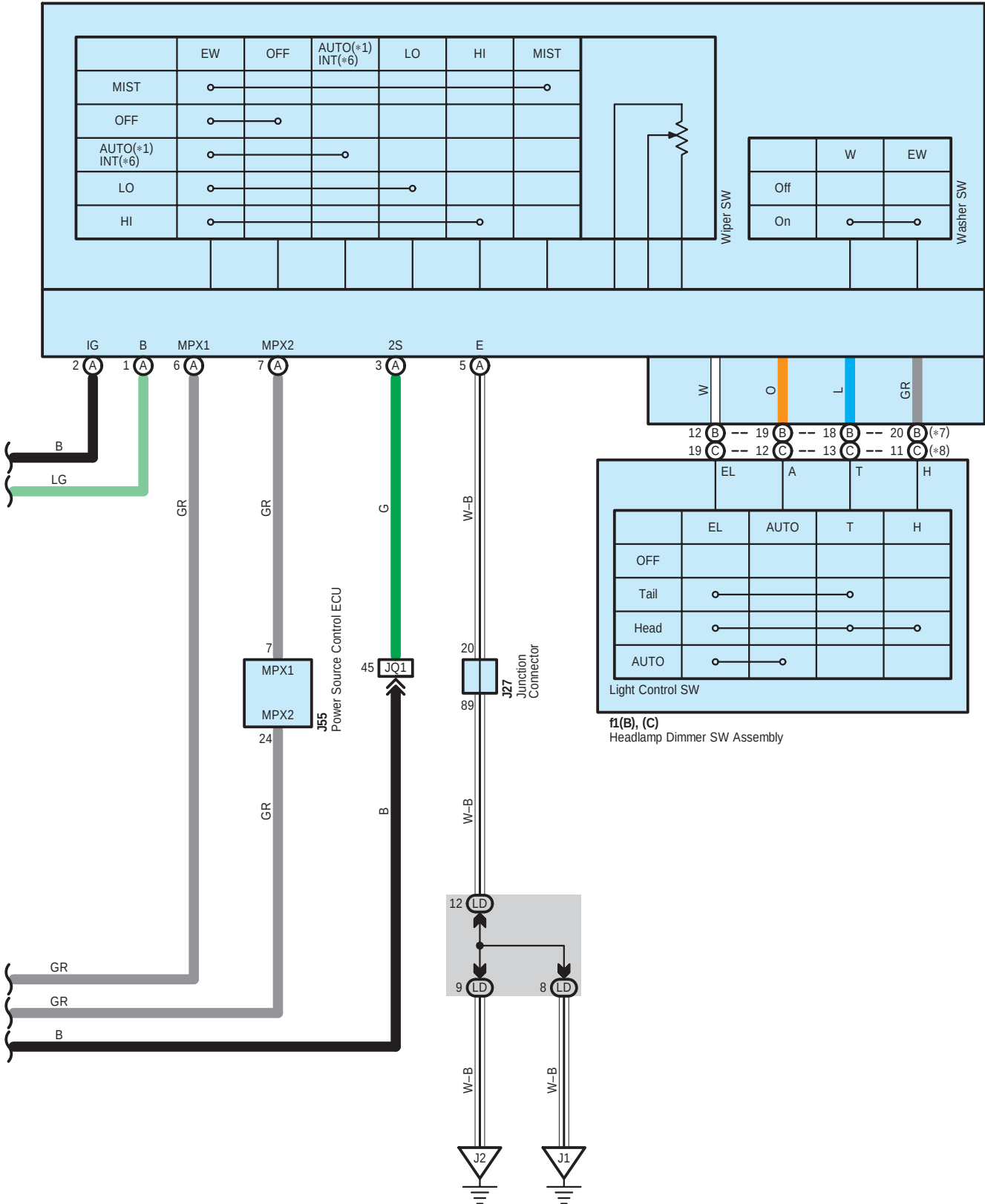
J26(A), f1(B), (C) Windshield Wiper SW Assembly
