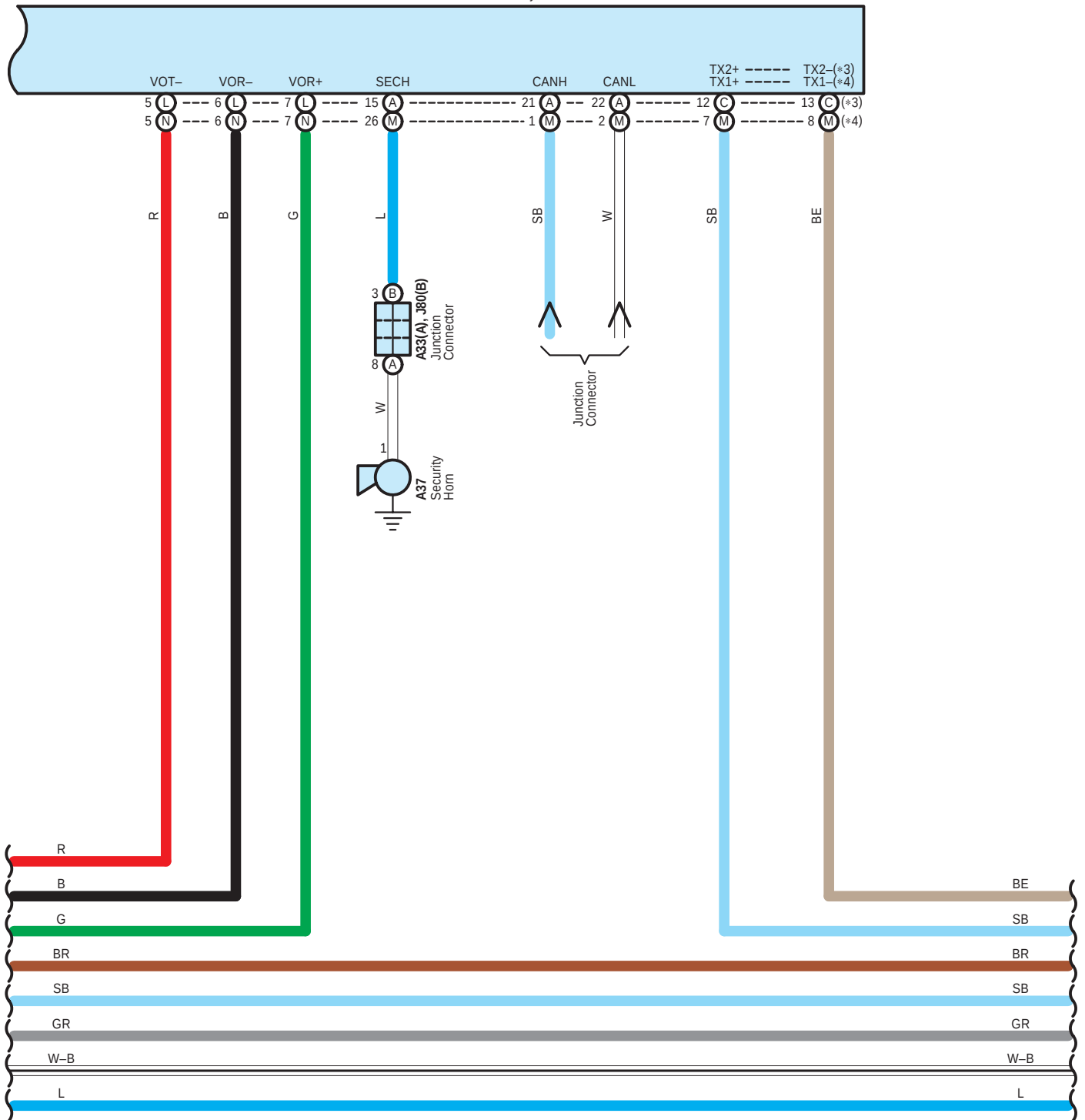
J122(A), J124(C), J134(L) Display & Navigation Module Display J140(M), J142(N) Multi-Media Module Receiver Assembly
