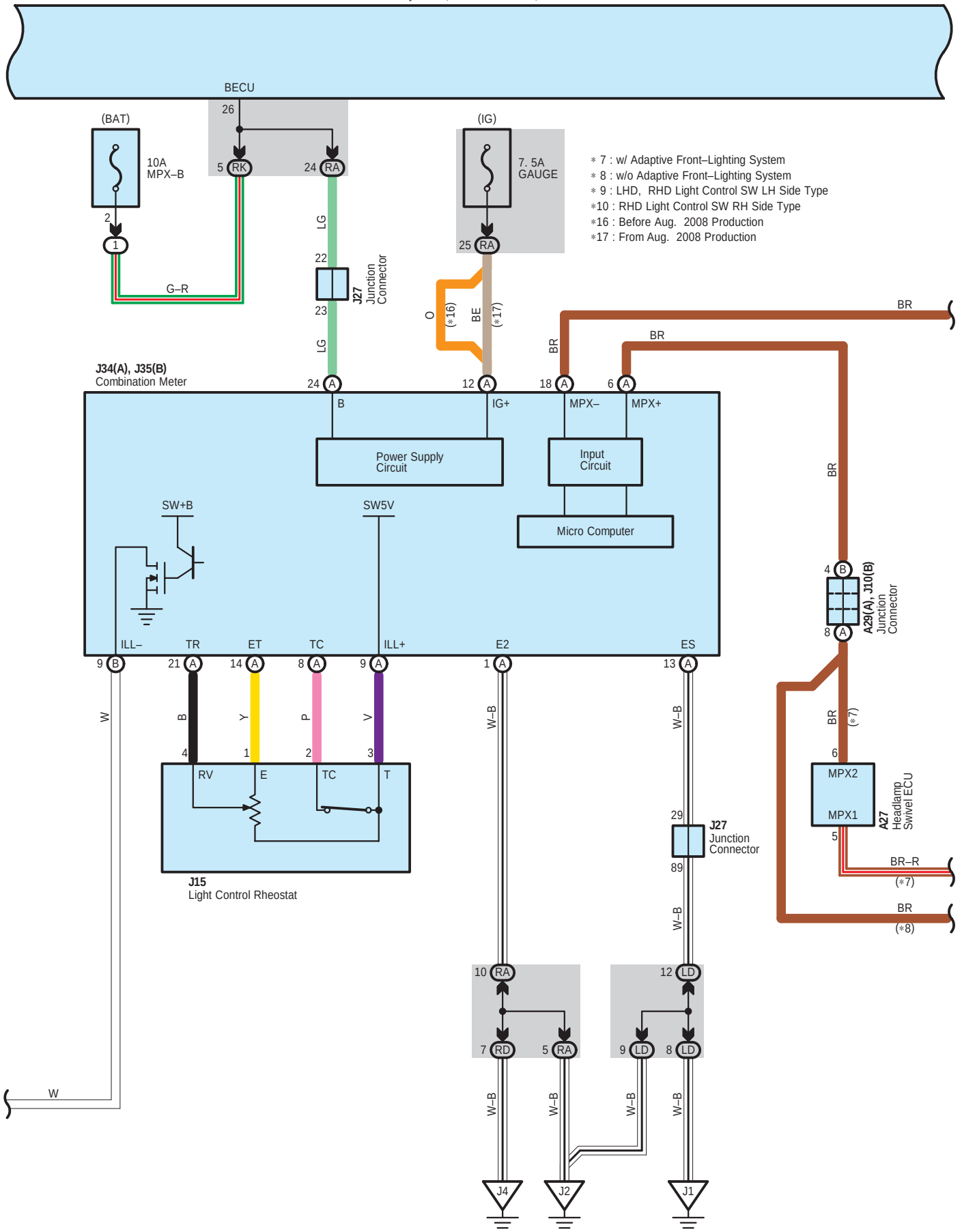
J75(B) Body ECU (Cowl Side J/B RH)
