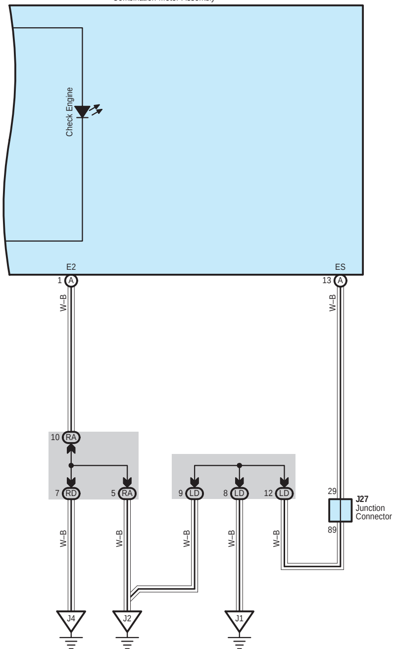
J34(A), J35(B) Combination Meter Assembly
