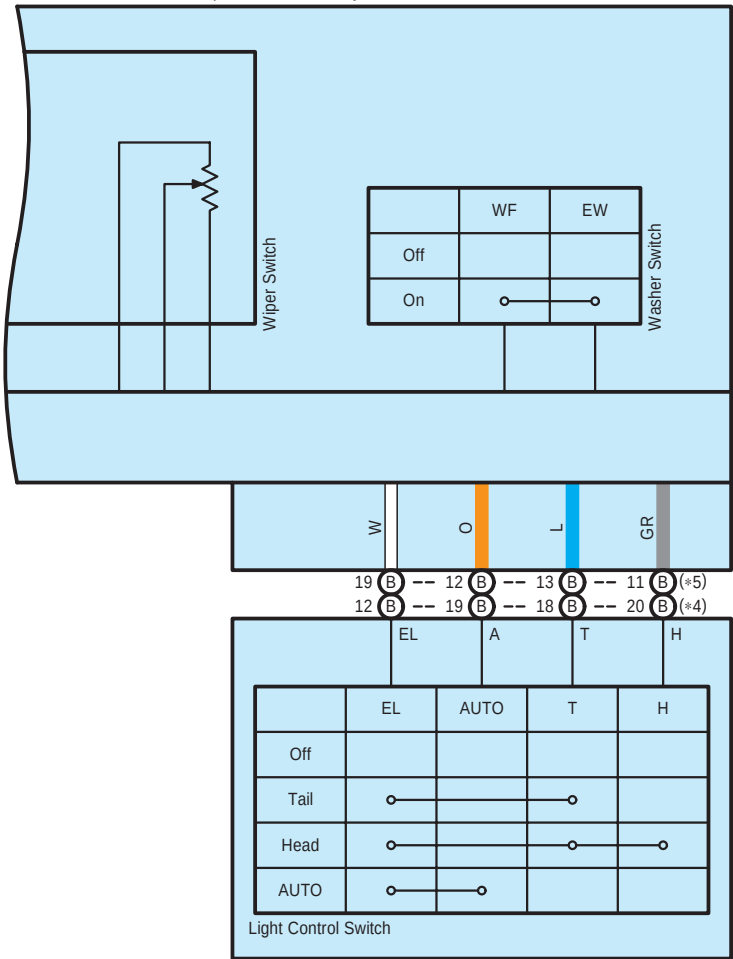
z4(B) Headlight Dimmer Switch Assembly
