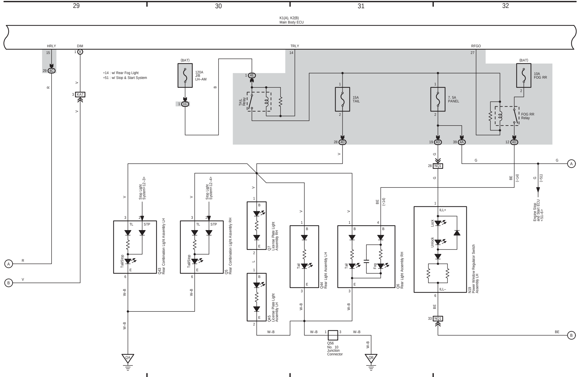
Taillight (RHD) (From Oct. 2016 Production)
