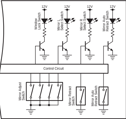
N3 Multiplex Network Master Switch Assembly
