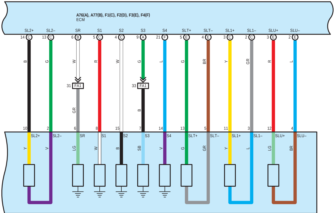
F56 ECT Solenoid (Transmission Wire)
