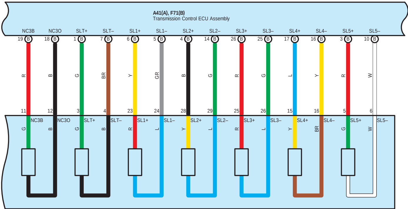
F73 ECT Solenoid (Transmission Wire)
