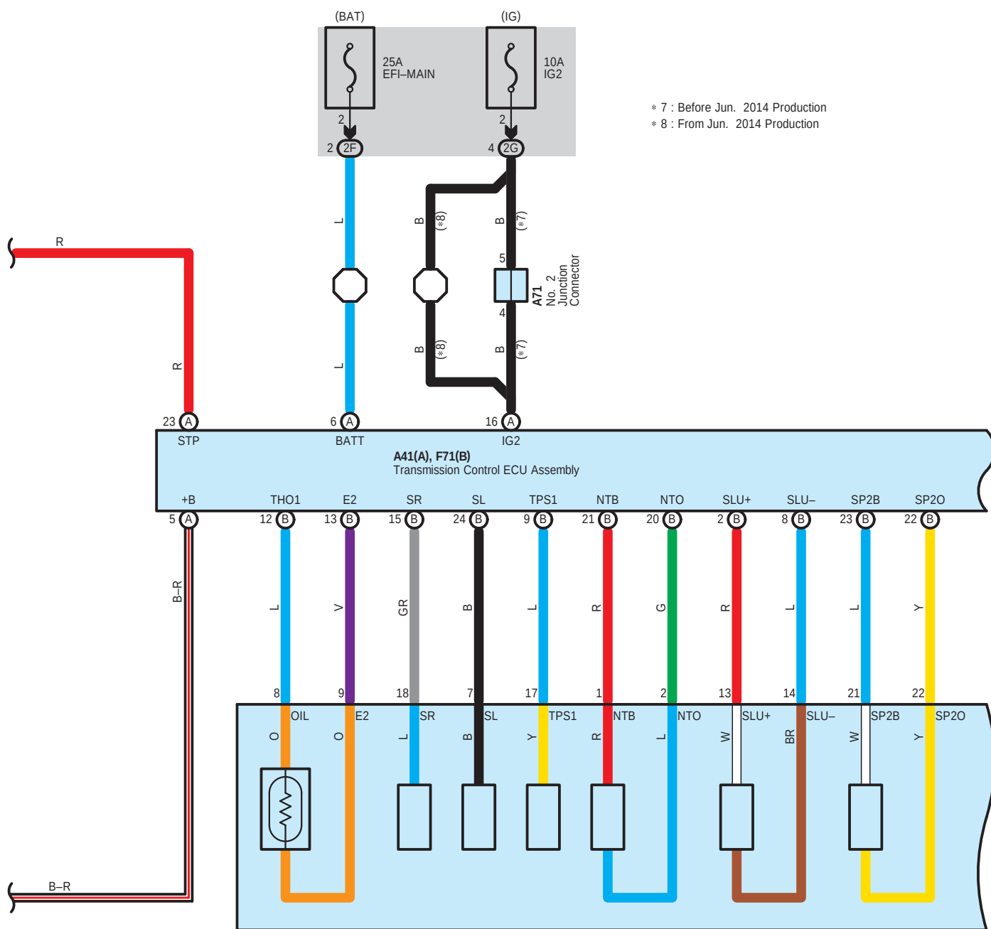
F73 ECT Solenoid (Transmission Wire)
