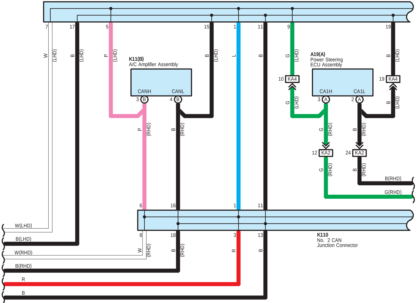
K109 No. 1 CAN Junction Connector
