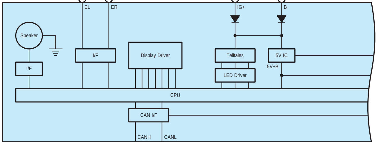
K3(A), K4(B) Combination Meter Assembly
