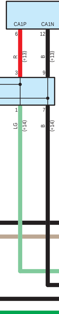
S9 Lane Departure Warning Camera
