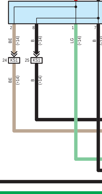
S17 No. 11 Junction Connector
