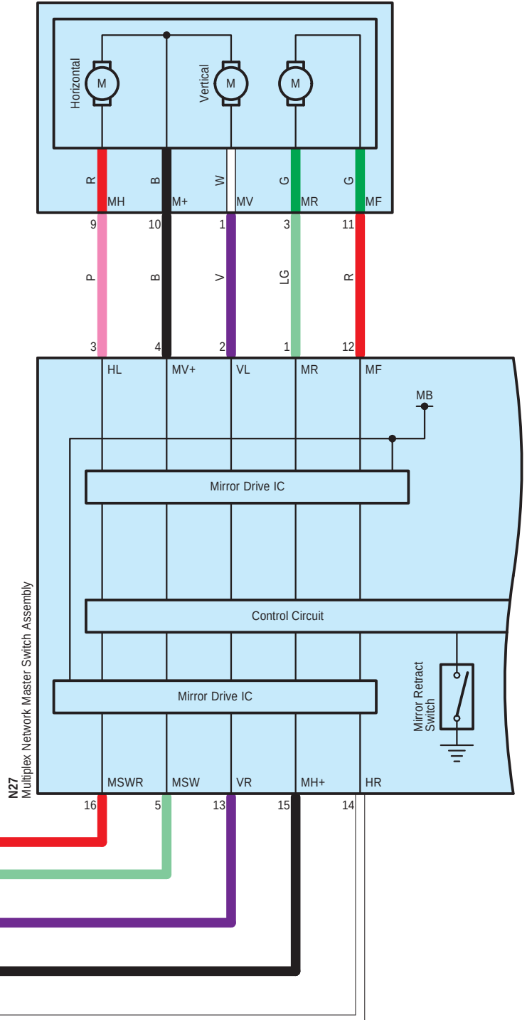
N23 Outer Rear View Mirror Assembly LH
