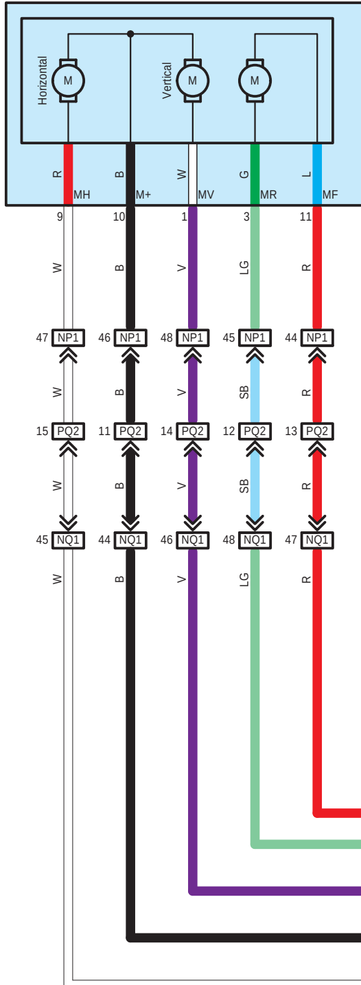
N8 Outer Rear View Mirror Assembly RH
