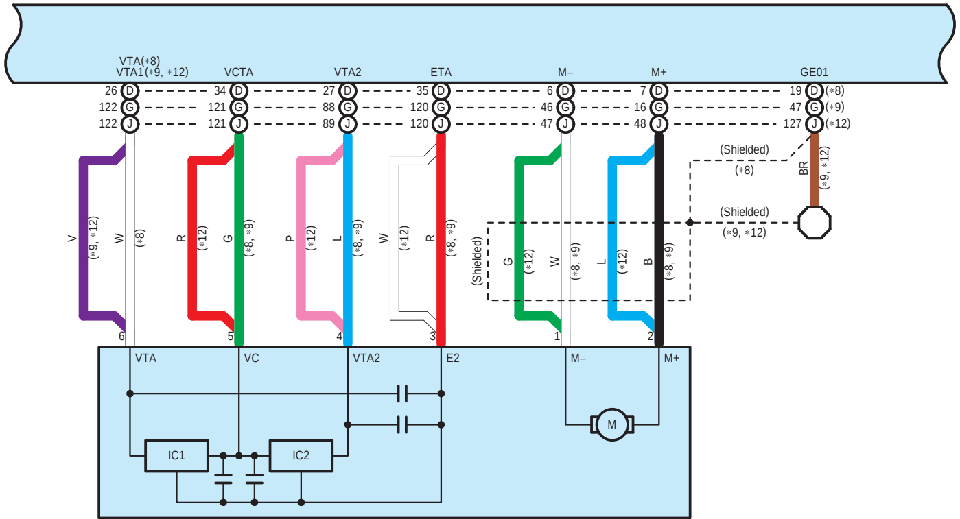
F21 Throttle Body with Motor Assembly
