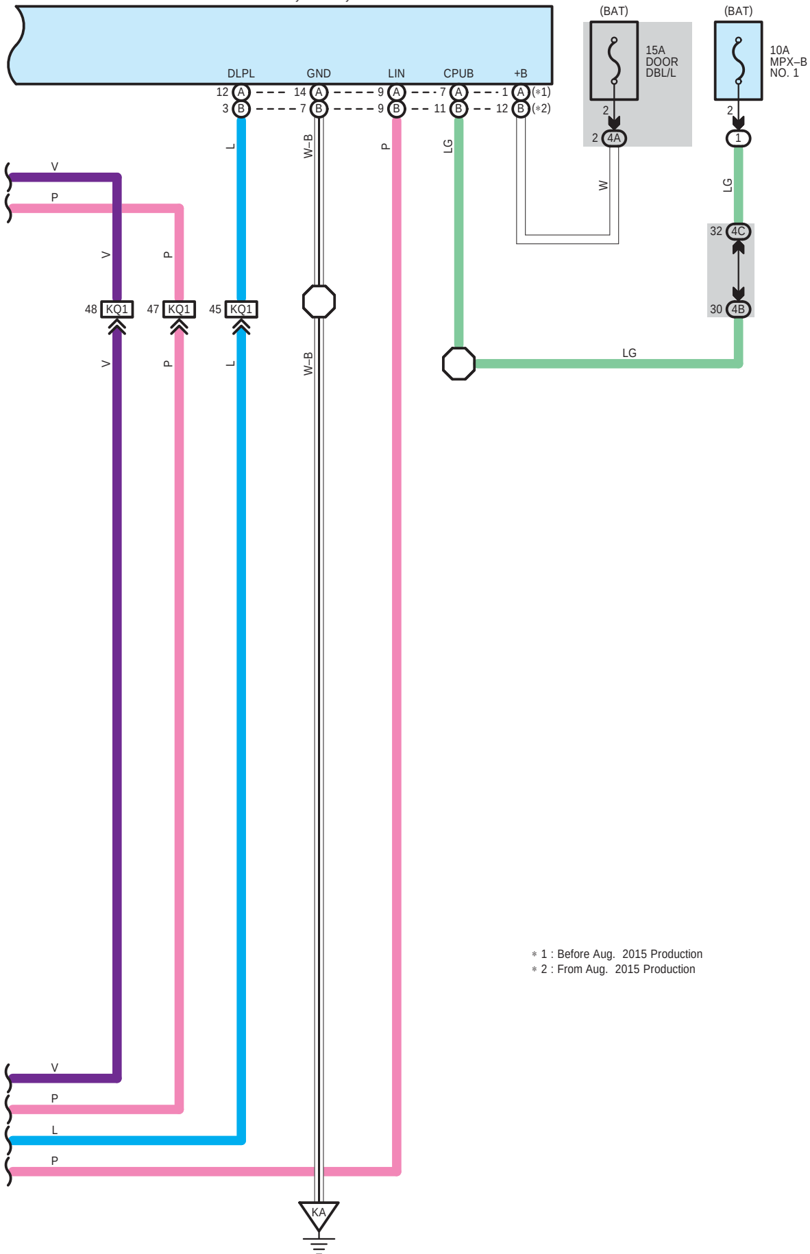
K42(A), K138(B) Double Lock Door Control Relay Assembly
